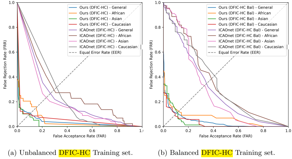
Fig. 11: Detection Error Tradeoff (DET) curves computed across a range of acceptance thresholds for different models and training sets, specifically: a) Ours and ICAOnet trained on the original DFIC-HC; and b) Ours and ICAOnet trained on a balanced version of DFIC-HC. All the combinations were tested on the same DFIC-HC sub-test sets (Protocol 3).
