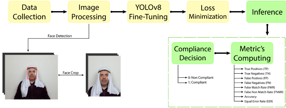
Fig. 6: A proposal of our methodology's sequential pipeline. All the images in the dataset are pre-processed before fine-tuning and further deploying of the model. This pre-process includes a facial detection stage that produces the bounding box (represented in red) that then serves as the base for a loose crop that produces the token frontal photo on the right. This crop's intention is to reproduce a real world scenario for a MRTD's portrait.
