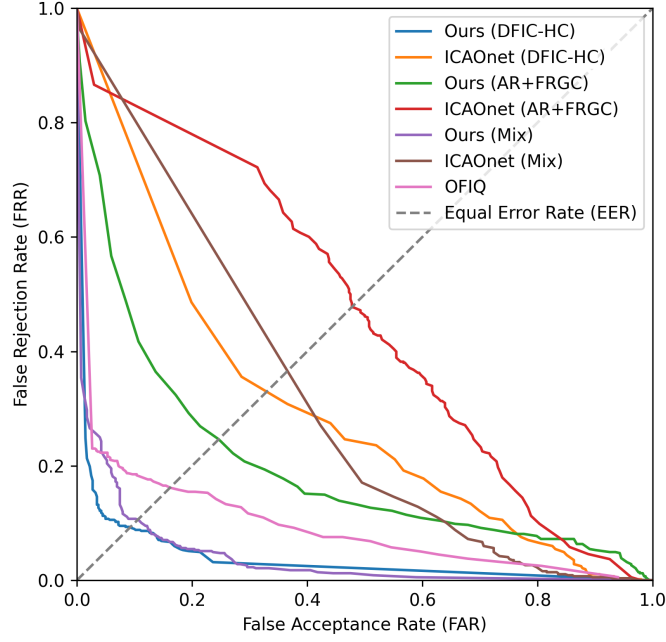
Fig. 10: Detection Error Tradeoff (DET) curves computed across a range of acceptance thresholds for different models and training sets. All the combinations were tested on the same Mixed test set ( Protocol 2.2 ).
