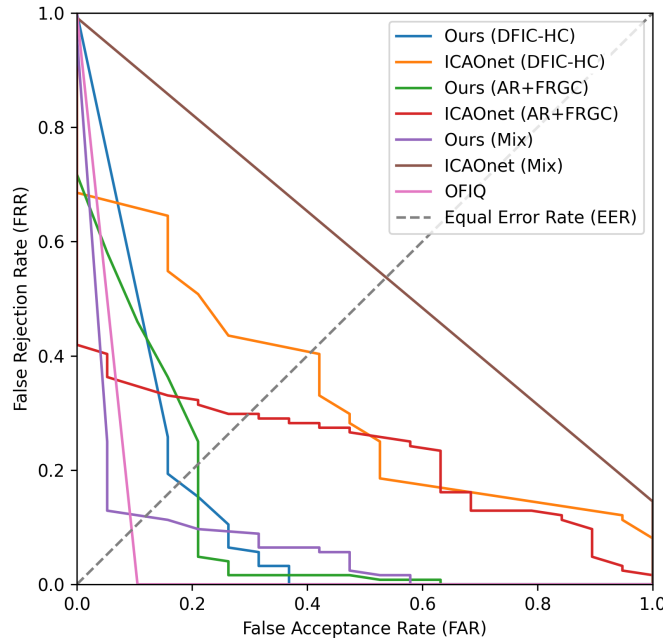
Fig. 9: Detection Error Tradeoff (DET) curves computed across a range of acceptance thresholds for different models and training sets. All the combinations were tested on the same AR+FRGC test set ( Protocol 2.1 ).
