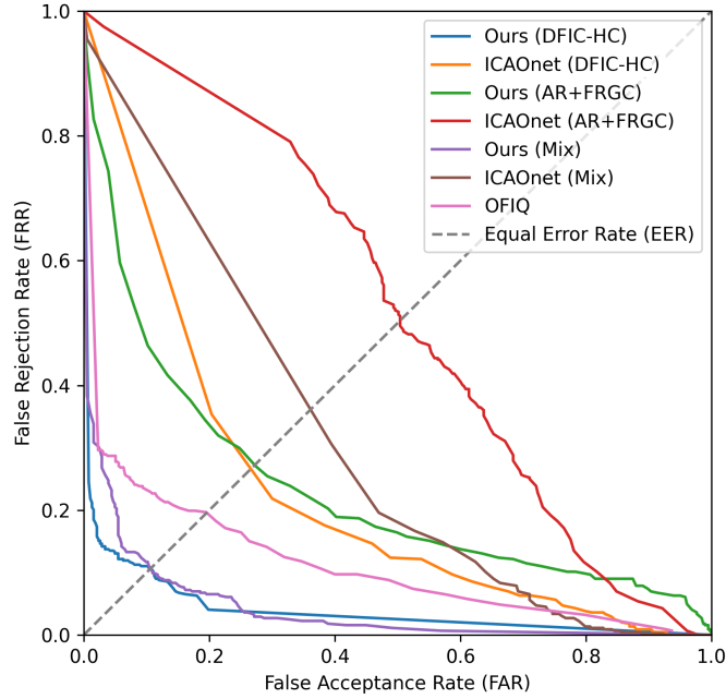
Fig. 8: Detection Error Tradeoff (DET) curves computed across a range of acceptance thresholds for different models and training sets. All the combinations were tested on the same DFIC-HC test set ( Protocol 1 ).
