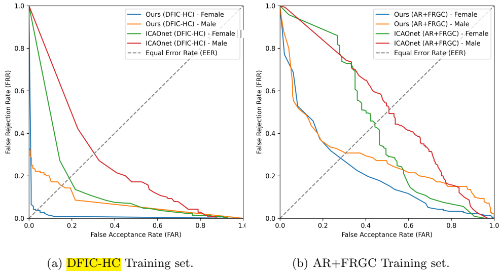
Fig. 14: Detection Error Tradeoff (DET) curves computed across a range of acceptance thresholds for different models and training sets, specifically: a) Ours and ICAOnet trained on DFIC-HC ; and b) Ours and ICAOnet trained on AR+FRGC. All the combinations were tested on the same DFIC-HC gender sub-test sets ( Protocol 4 (Gender) ).
