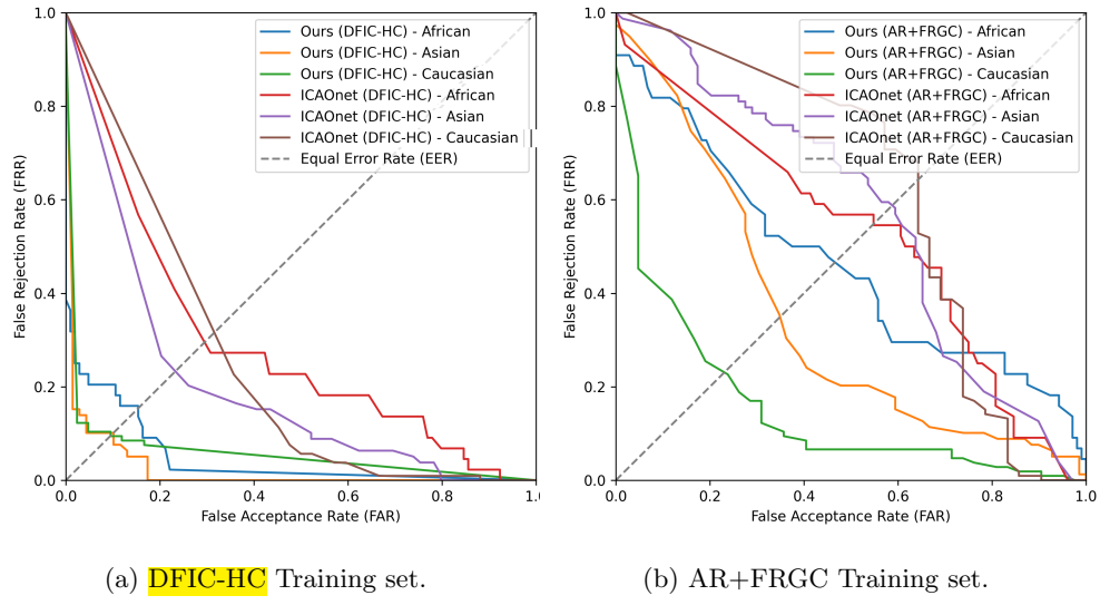
Fig. 13: Detection Error Tradeoff (DET) curves computed across a range of acceptance thresholds for different models and training sets, specifically: a) Ours and ICAOnet trained on DFIC-HC ; and b) Ours and ICAOnet trained on AR+FRGC. All the combinations were tested on the same DFIC-HC ethnicity sub-test sets ( Protocol 4 (Ethnicity) ).
